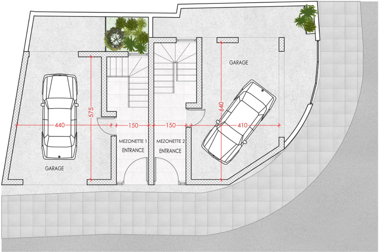
GROUND FLOOR
