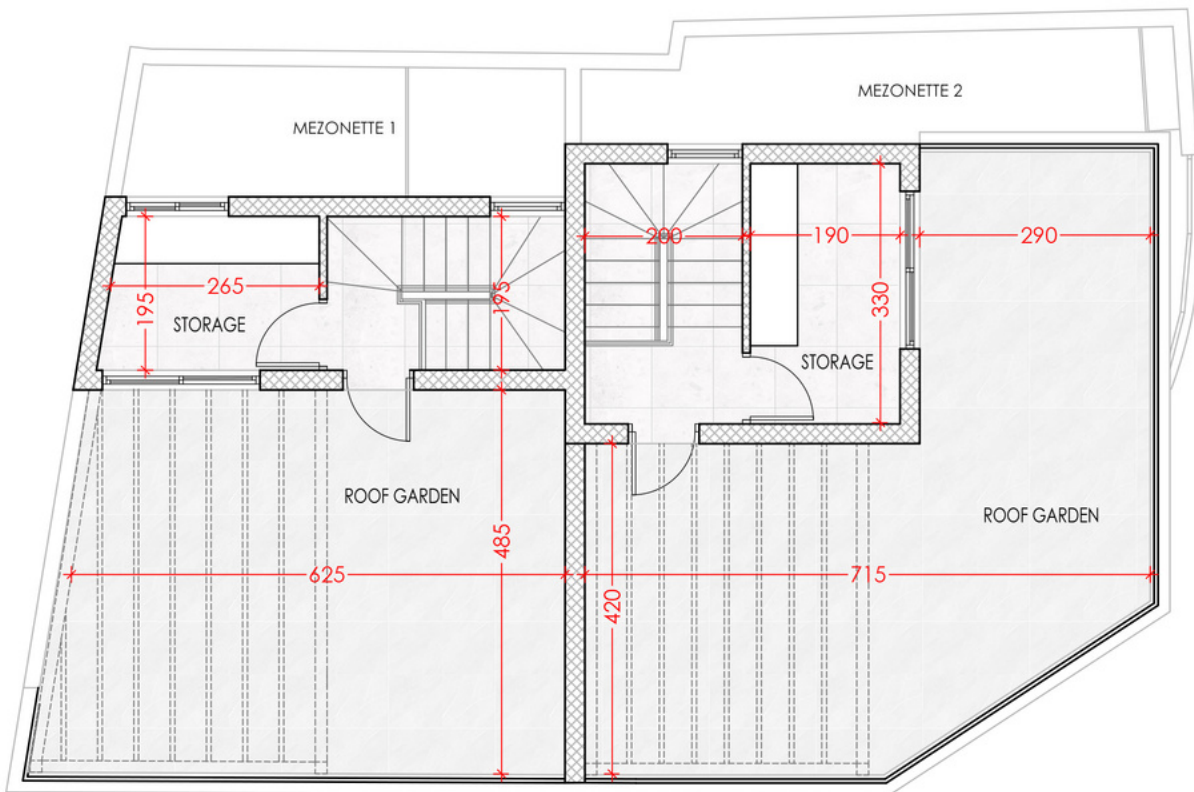
ROOF GARDEN
